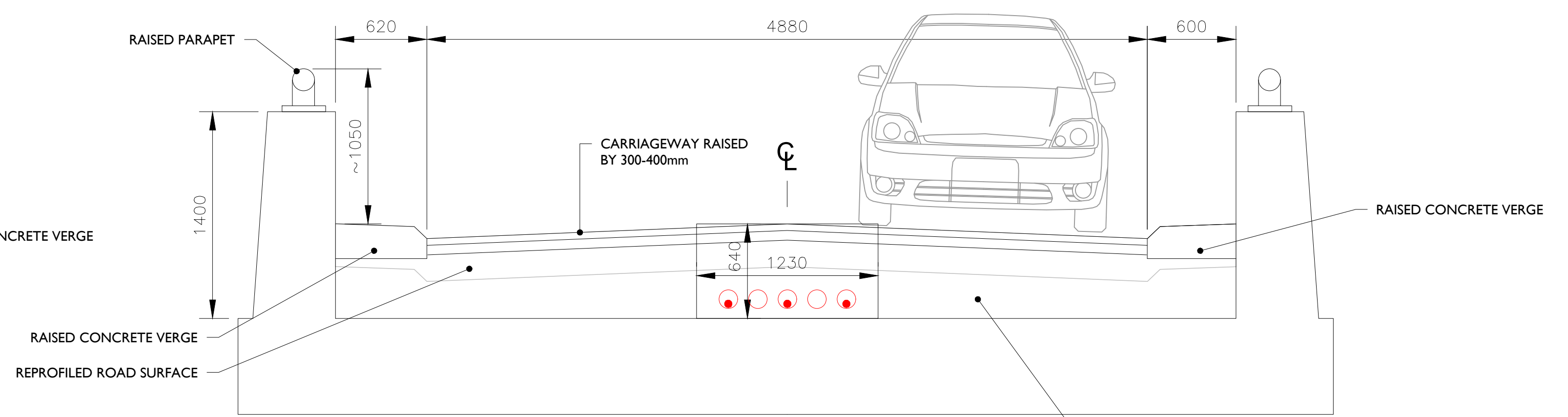
SECTION A-A - PROPOSED OPTION D DUCTS IN ROAD SCALE 1:25
